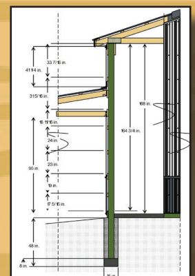
CROSS SECTION DETAILS
