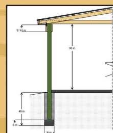
CROSS SECTION DETAILS
