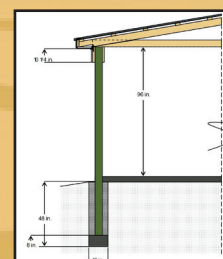
CROSS SECTION DETAILS
