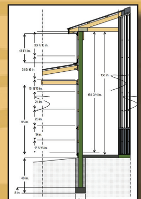
CROSS SECTION DETAILS
