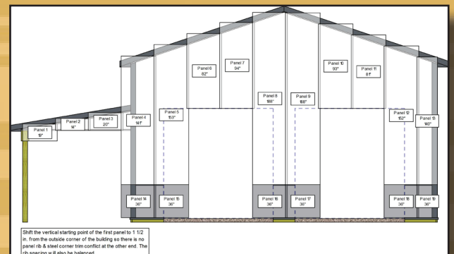
STEEL PANEL LAYOUTS
